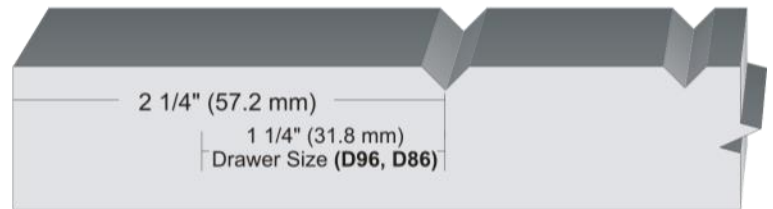
M96 V-Groove Panel & V-Groove Through Stile and Rail
