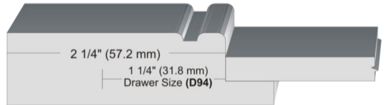
M94 2 pc. Recessed Panel Beaded Stile and Rail
