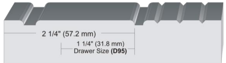
M95 Beaded (Washboard) Raised Panel
