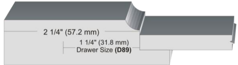
M89 2 pc. Cove Recessed Panel
