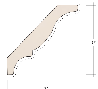
1025-TRAD CROWN Core: MDF Wrapped Surface
